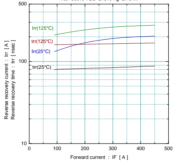
Reverse recovery characteristics (typ.) V_{CC}=600\text{V} , V_{GE}=\pm 15\text{V} , R_g=2.7\Omega\text{m}
