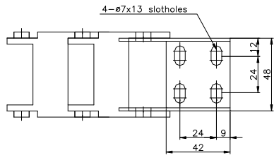
VIEW-C MOVING END (S=1.5:1)
