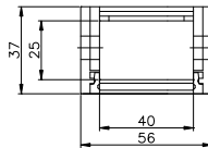
SECTION A-A (S=1.5:1)
