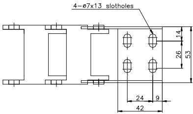
VIEW-B FIXED END (S=1.5:1)
