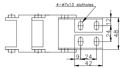
VIEW-C MOVING END (S=1.5:1)
