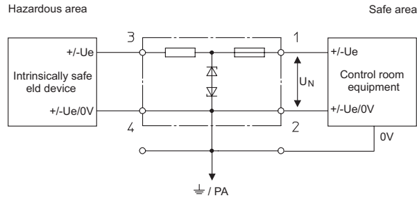
Single-Channel Safety Barriers for Alternating Polarity
