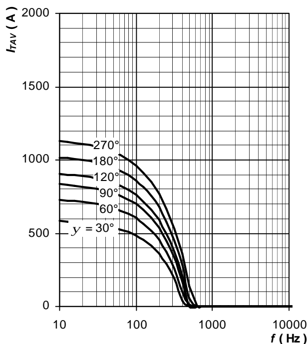
Fig. 35 Average on-state current vs. frequency, trapezoid waveform, T_C = 90\text{ }^\circ\text{C} , di_T/dt = \pm 500\text{ A}/\mu\text{s} , V_R = 2/3\text{ }V_{DRM}
