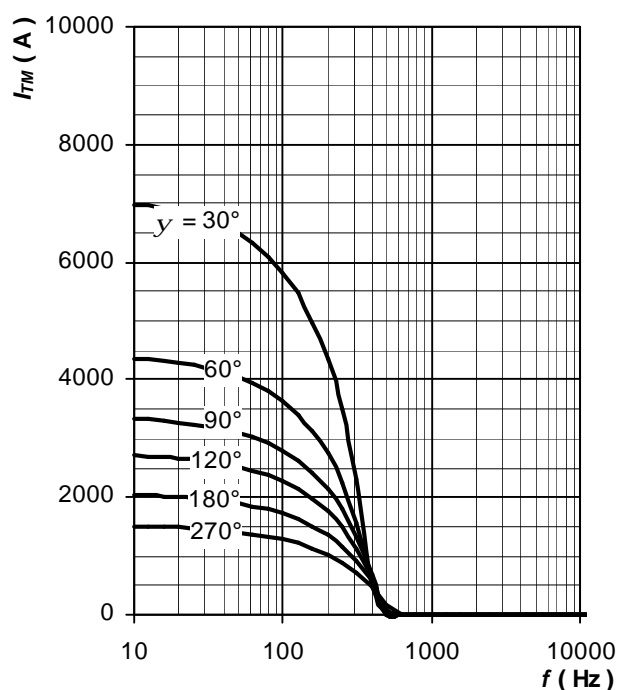
Fig. 36 Maximum on-state current vs. frequency, trapezoid waveform, T_C = 90\text{ }^\circ\text{C} , di_T/dt = \pm 500\text{ A}/\mu\text{s} , V_R = 2/3\text{ }V_{DRM}
