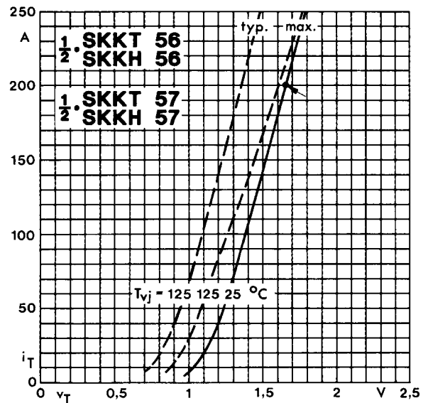
Fig. 8 On-state characteristics
