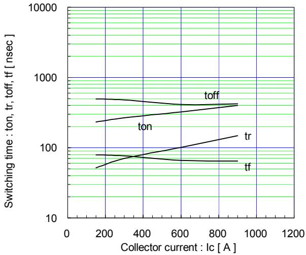
Switching time vs. Collector current (typ.) V_{CC}=600V, V_{GE}=\pm 15V, R_G=1.1\Omega, T_J=25^\circ C
