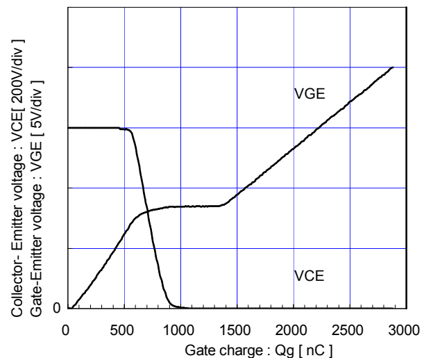
Dynamic Gate charge (typ.) Vcc=600V, Ic=600A, Tj=25°C
