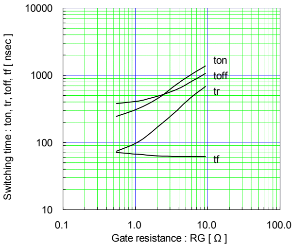
Switching time vs. Gate resistance (typ.) V_{CC}=600V, I_C=600A, V_{GE}=\pm 15V, T_J=25^\circ C
