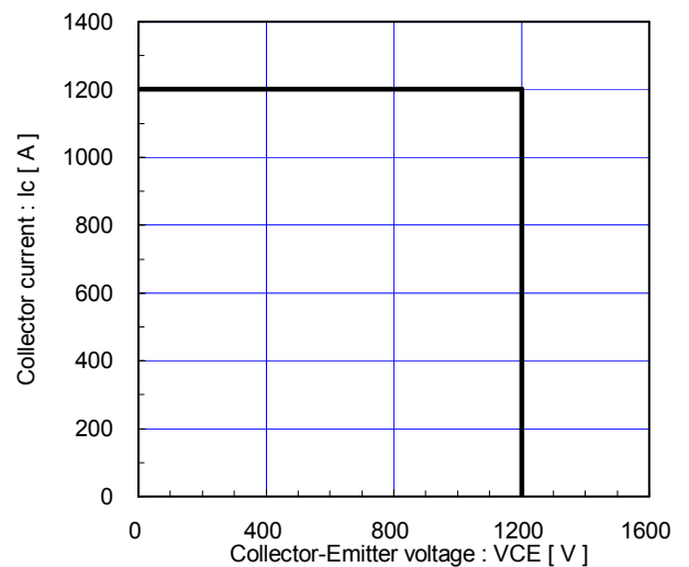
Reverse bias safe operating area (max.) +V_{GE}=15V, -V_{GE} \le 15V, R_G \ge 1.1\Omega, T_J \le 125^\circ C
