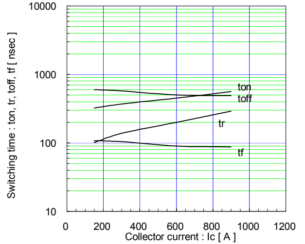
Switching time vs. Collector current (typ.) V_{CC}=600V, V_{GE}=\pm 15V, R_G=1.1\Omega, T_J=125^\circ C
