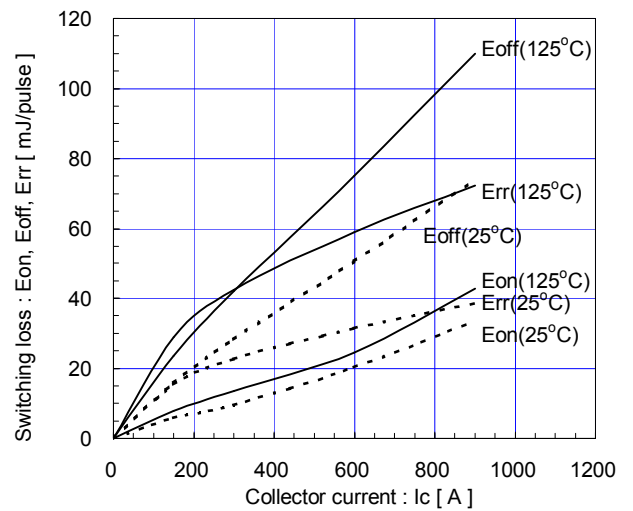
Switching loss vs. Collector current (typ.) V_{CC}=600V, V_{GE}=\pm 15V, R_G=1.1\Omega
